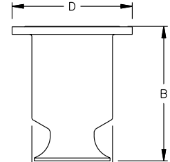
120° Flanged
